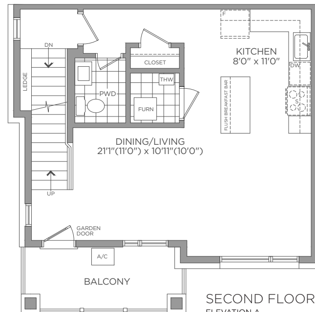
OPT. SECOND FLOOR ELEVATION A
