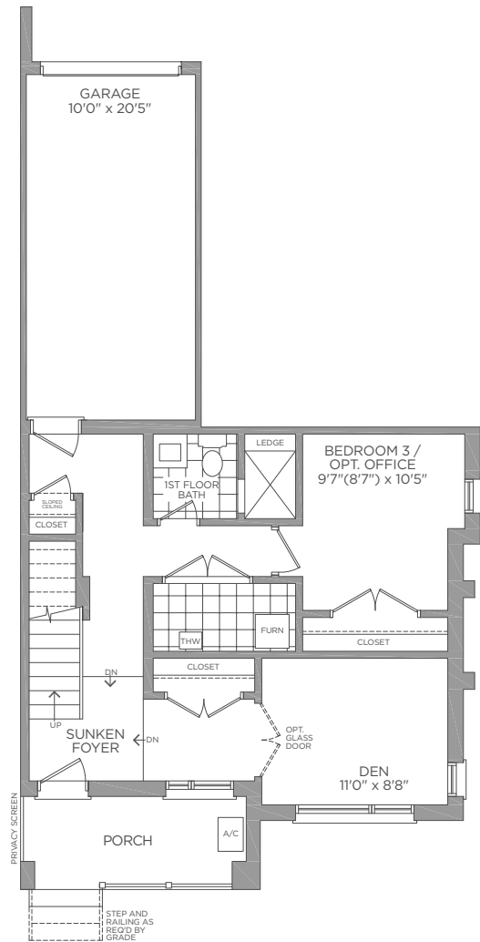
FIRST FLOOR ELEVATION A BLOCK F - UNIT 74
