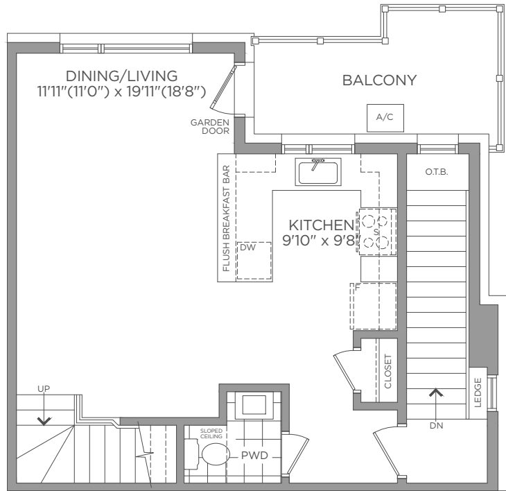
SECOND FLOOR ELEVATION A BLOCK F - UNIT 73 ONLY
