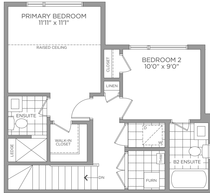
OPT. THIRD FLOOR ELEVATION A BLOCK F - UNIT 73 ONLY
