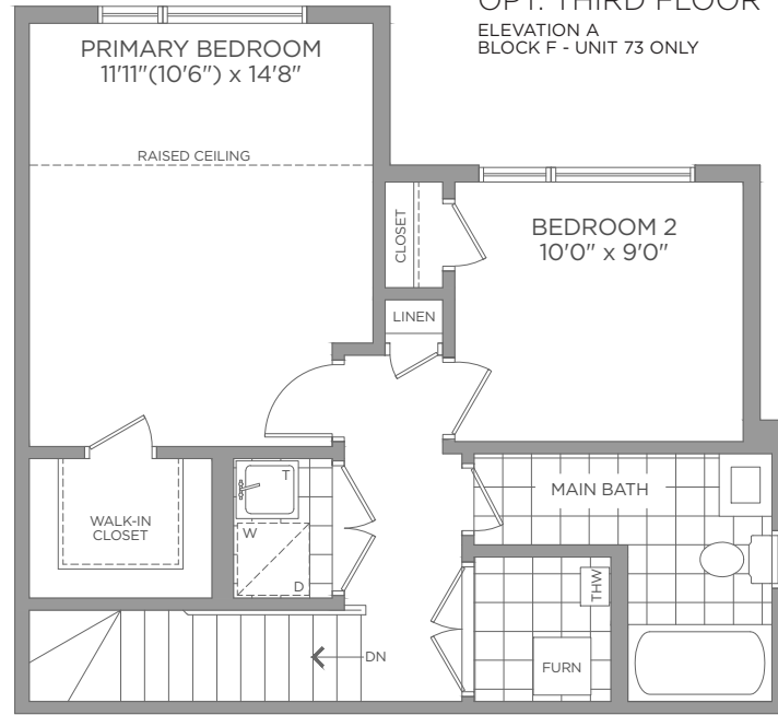
THIRD FLOOR ELEVATION A BLOCK F - UNIT 73 ONLY
