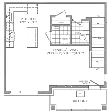
SECOND FLOOR ELEVATION A
