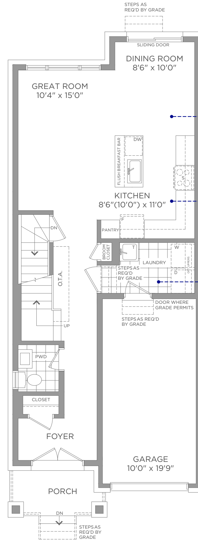
First Floor ELEVATION A, A(V)
