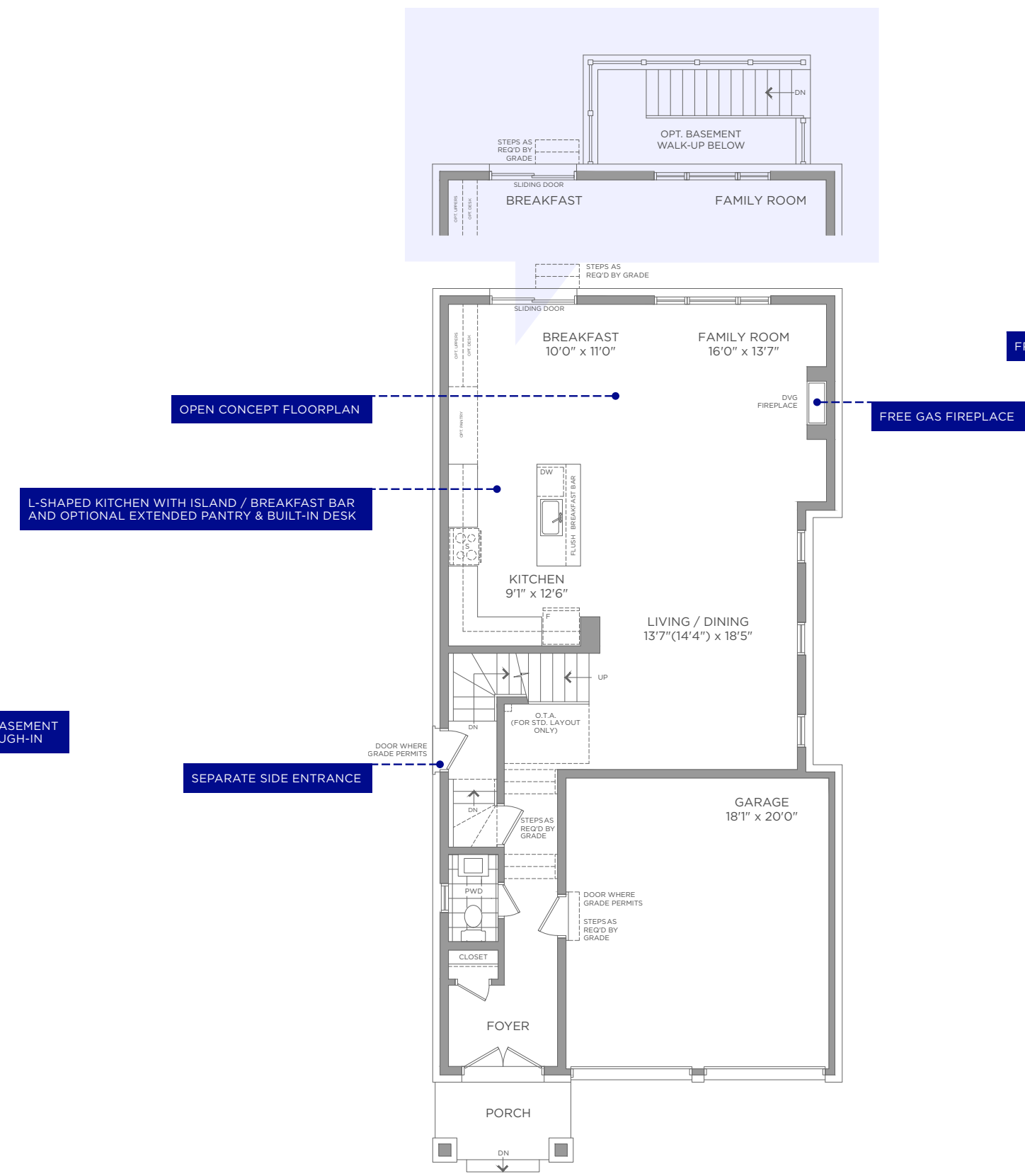
FIRST FLOOR WITH OPT. WALK UP ELEVATION A, A(V)
