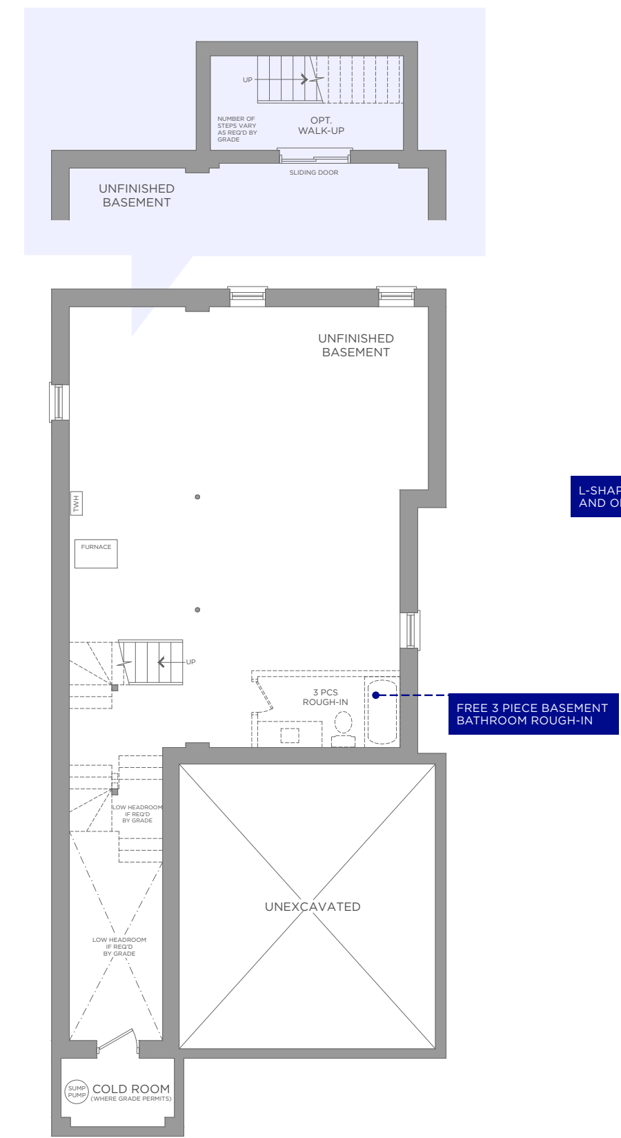
BASEMENT WITH OPT. WALK UP ELEVATION A, A(V)
