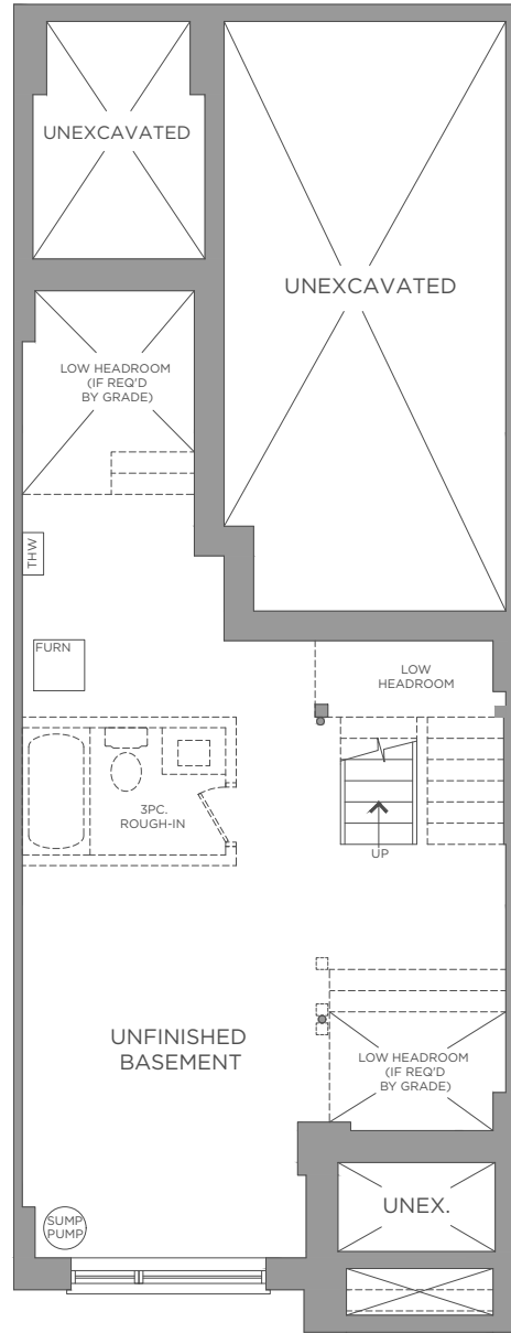
BASEMENT ELEVATION A
