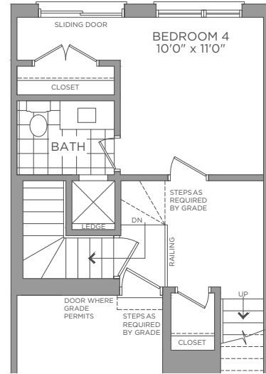
OPT. FIRST FLOOR ELEVATION A / B
