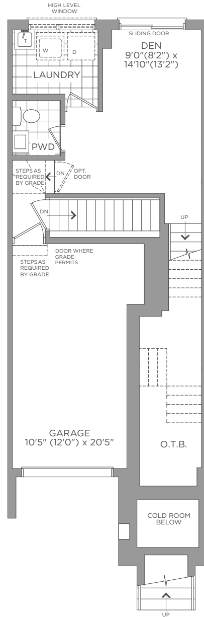
FIRST FLOOR ELEVATION A / B
